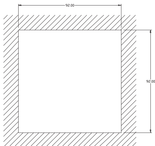
Mechanical dimensions and front panel cutout (mm)
